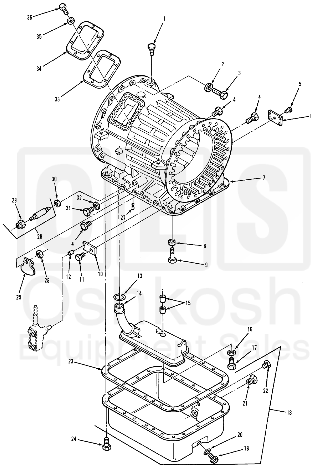
FIGURE 65. TRANSMISSION HOUSING.
